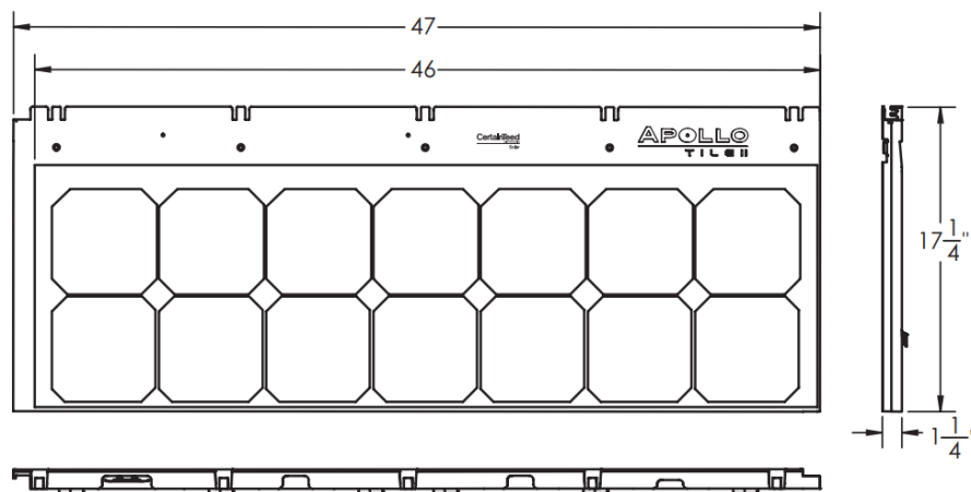
Figure 1: Apollo II Tile Dimensions
