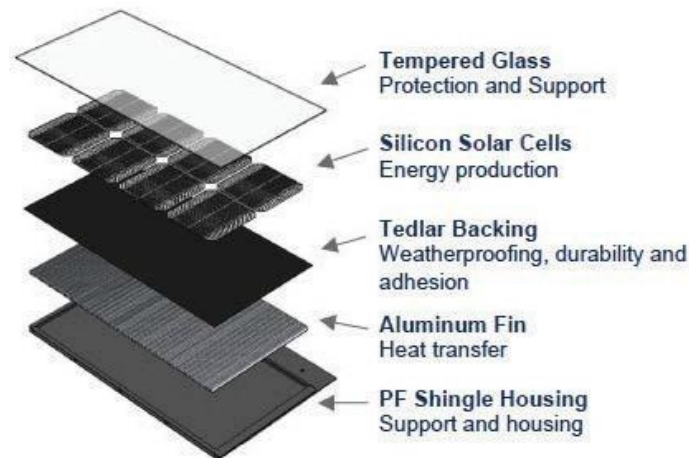
Figure 2: Solar Shingle Assembly
