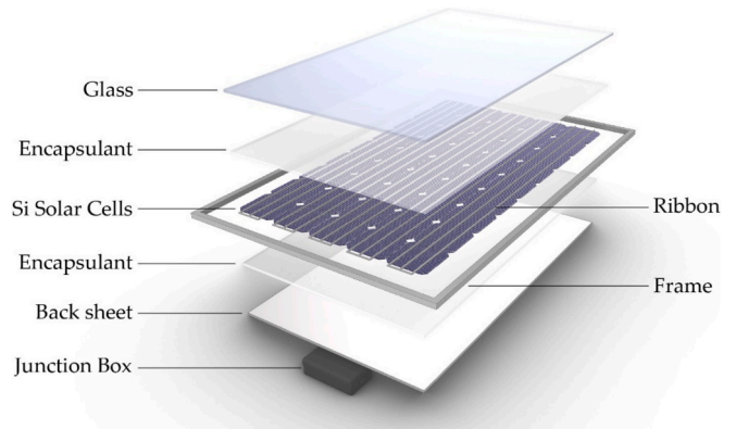
Fig. 5. Structure of a silicon-based solar PV module. ([], open access). Source: 45
