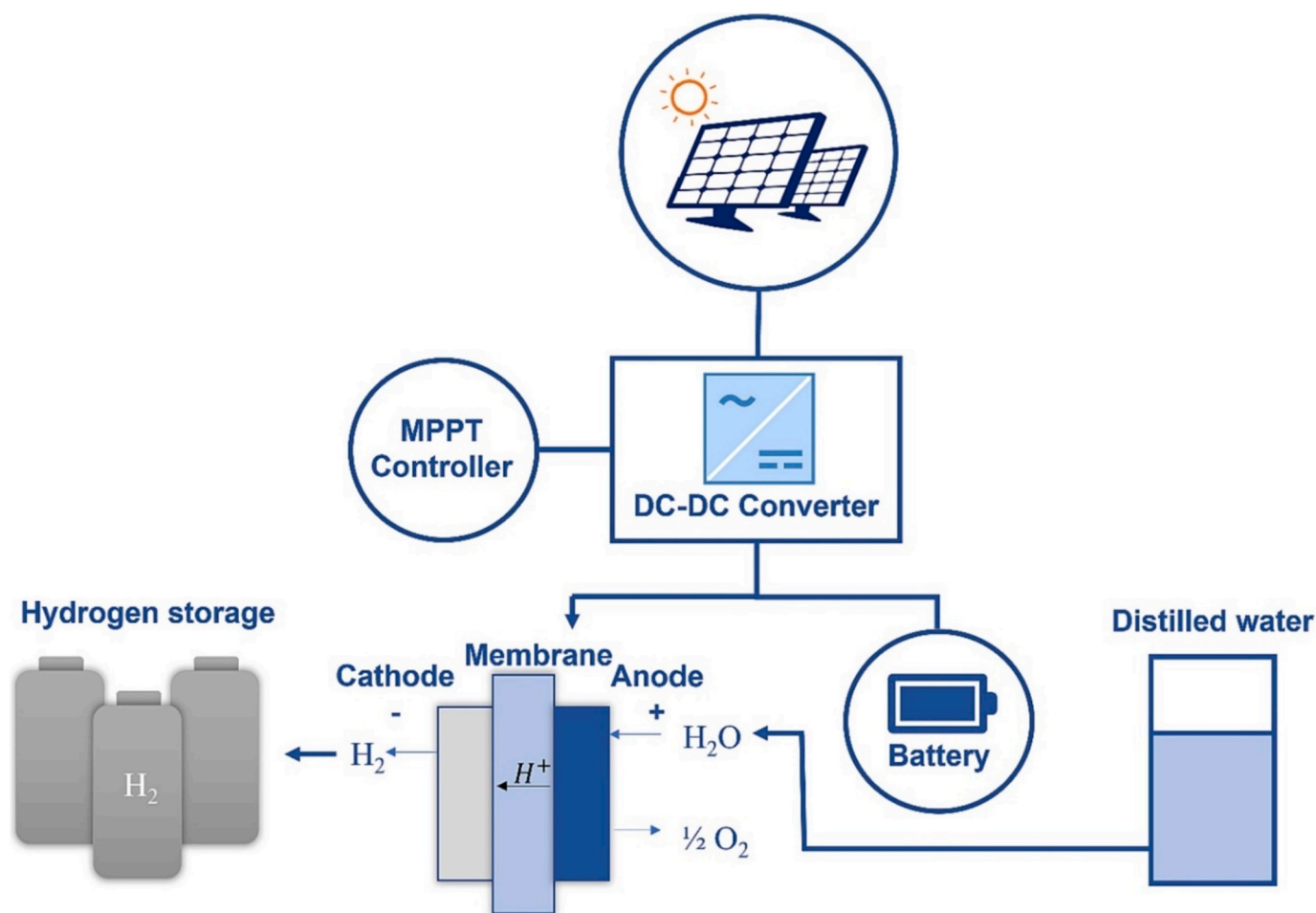
Fig. 11. Schematic diagram of a photovoltaic-driven hydrogen production system. ([], with permission number 5931390106178).
