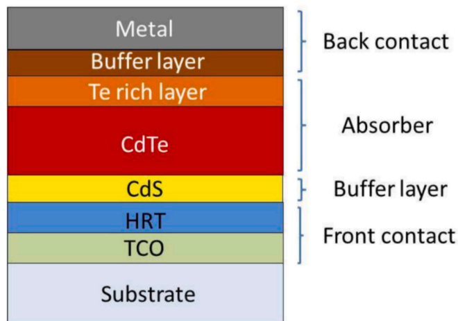
Fig. 6. Structure of a cadmium telluride solar cell. ([], open access). Source: 49
