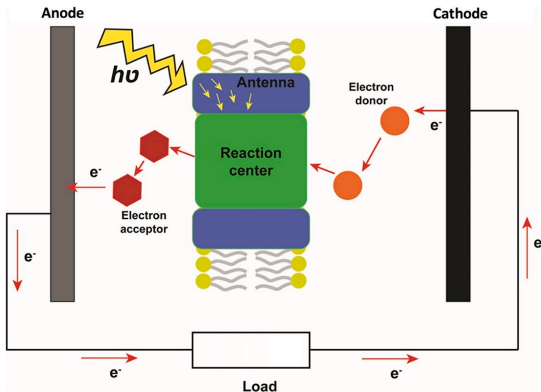
Fig. 9. Schematic diagram of a biohybrid solar cell's operation. ([], with permission number 5932310089785).
