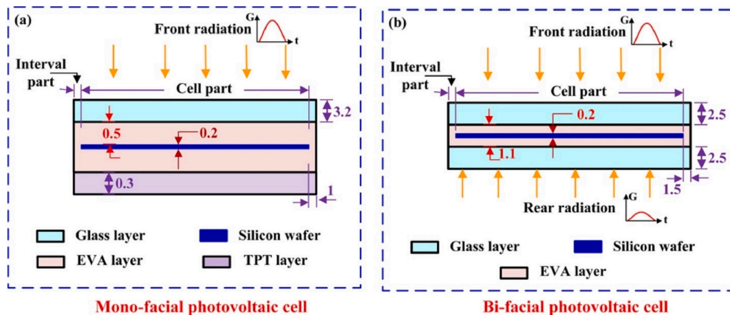
Fig. 10. Schematic diagram of (a) mono-facial and (b) bi-facial PV panels. ([], open access). Source: 92
