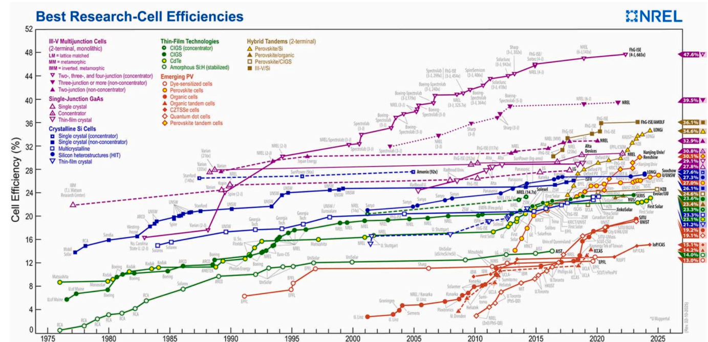
Fig. 4. The highest confirmed conversion efficiencies for research cells for a range of photovoltaic technologies. ([], open access). Source: 41
