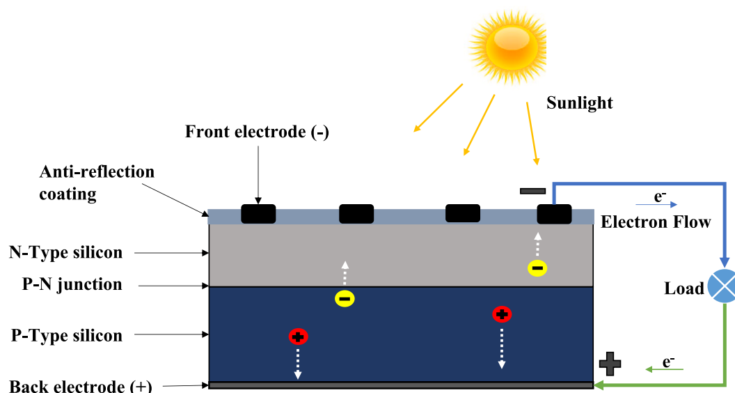
Fig. 1. Schematic diagram of a photovoltaic cell.
