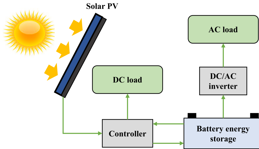
Fig. 2. Stand-alone solar PV system layout.
