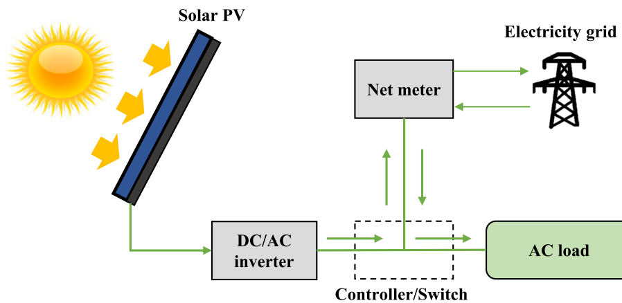
Fig. 3. Grid-tied solar PV system layout.
