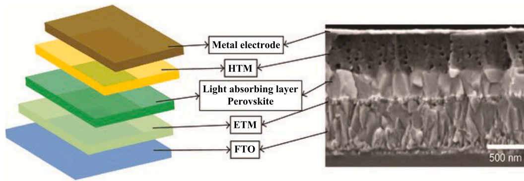
Fig. 7. Structure of a perovskite solar cell. ([], open access). Source: 61
