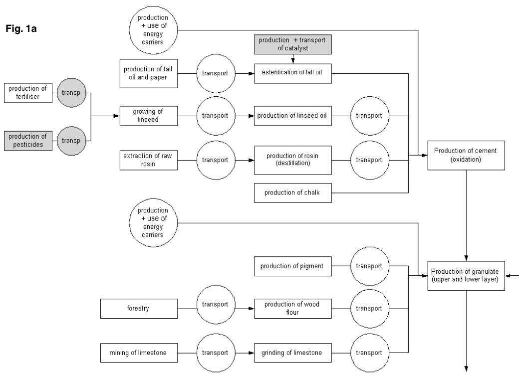
Fig. 1: Process tree for the use and disposal of linoleum floors. The production of capital goods is excluded from the system.
