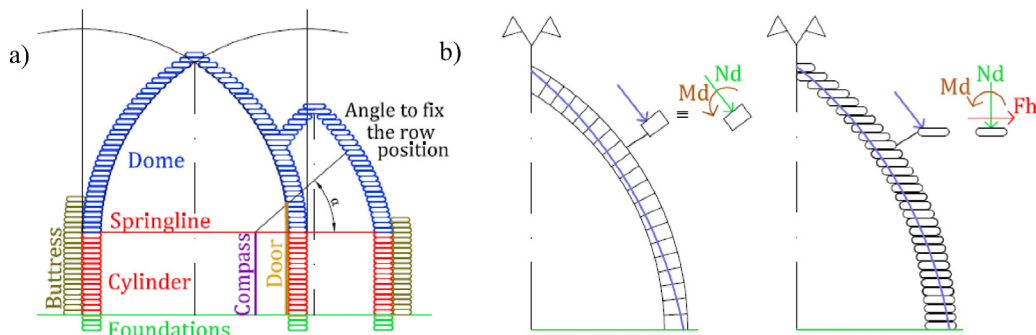
Fig. 2. Cross section of a dome house (a) conventional and superadobe domes differences (b).
