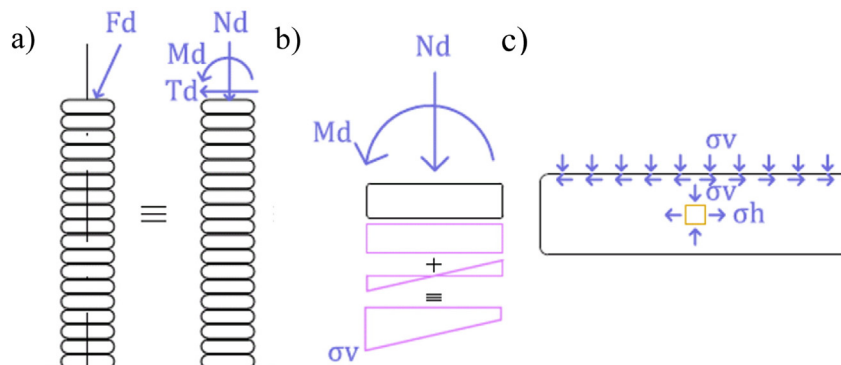
Fig. 3. Forces N_d , T_d and M_d acting on the wall (a), combined bending and axial compression in a row (b), stresses in a bag under vertical loading (c).
