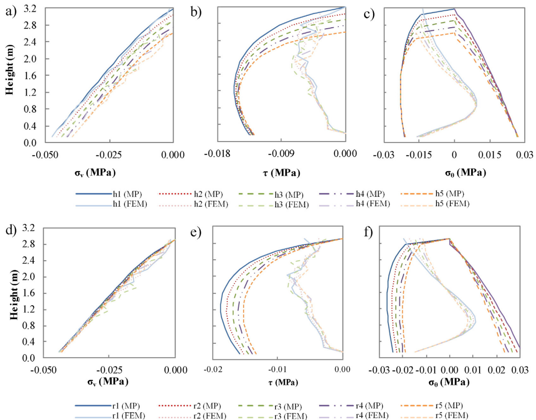
Fig. 11. Comparison of vertical ( \sigma_v ), shear ( \tau ) and hoop stress ( \sigma_\theta ) computed by MP and FEM for different curvatures: varying the height (a, b, c) and varying the radius curves (d, e, f).
