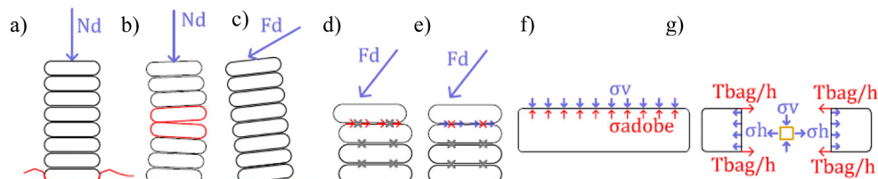
Fig. 4. Possible failure mechanisms: global collapse (a), buckling (b), roll-over (c), local slipping (d), tear of the bag (e), adobe failure (f) and bag failure (g).
