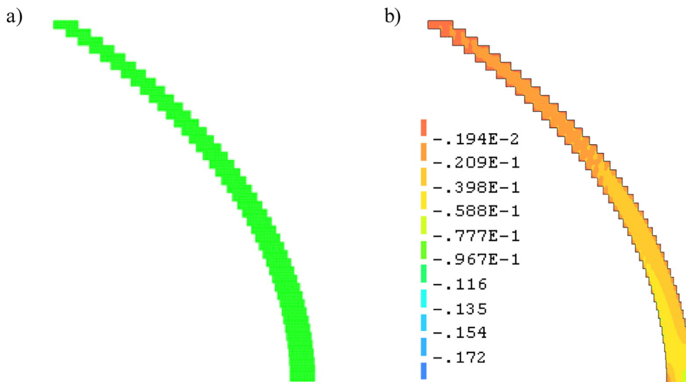
Fig. 9. Mesh used in the study (a) typical stress distribution in MPa in the vertical direction (b).
