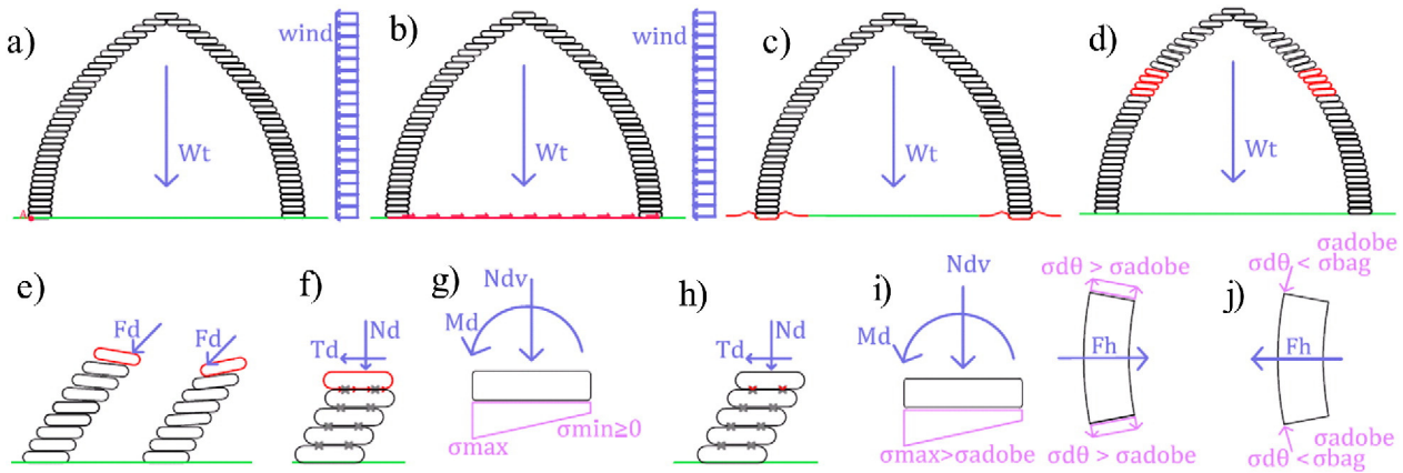
Fig. 8. Failure schemes according to Table 5 (Eqs. (39)–(51)): Global roll-over (a), global slipping (b), collapse (c), buckling (d), local roll-over (e), local slipping (f), vertical compression (g), tear of the bag (h), adobe failures (i) and bag or adobe failure in hoop direction (j).
