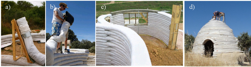
Fig. 1. Construction of superadobe structures (sources: www.labioguia.com (a), www.domoterra.es (b, d), www.earthbagbuilding.com (c)).
