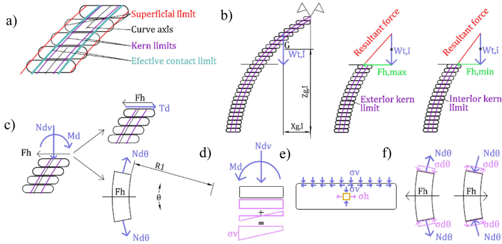
Fig. 7. Detail of the calculus limits domains (a), the resultant force must be inside of the kern limits (b), force equilibrium (c), distribution of vertical stresses along the adobe section (d), horizontal stresses (e) and hoop forces and stresses due to the radial force (f).
