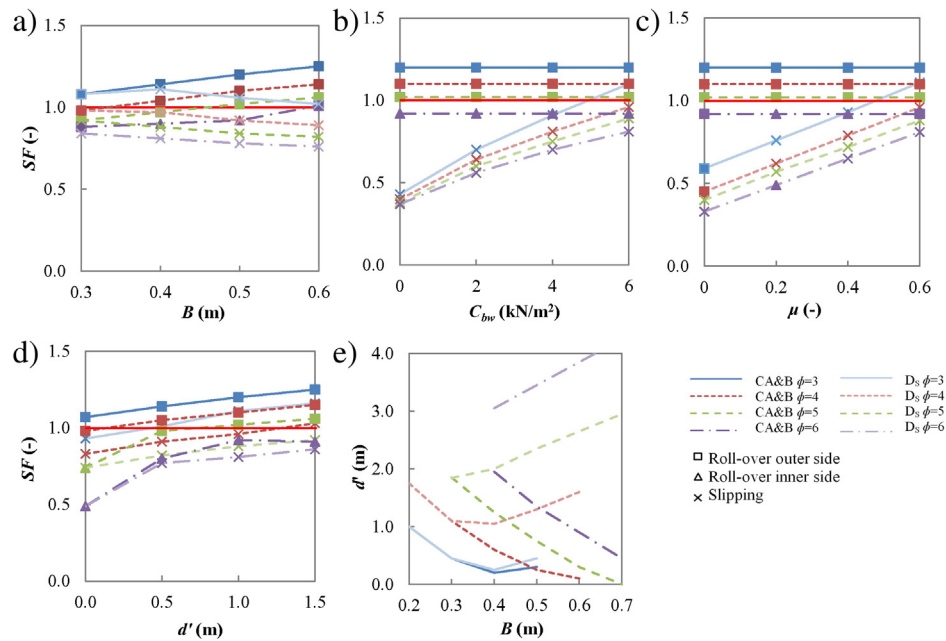
Fig. 13. Influence of the width of the bag (a), the cohesion of the interface (b), the friction coefficient between bags (c) and the curvature parameter (d) on the safety factor and the optimal design of the curvature parameter (e).
