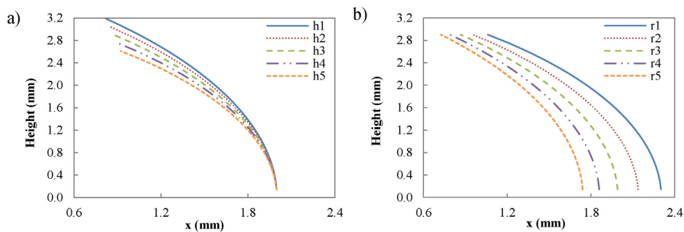
Fig. 10. Arches simulated: constant the radius and variable height (a), constant height and variable the radius (b).
